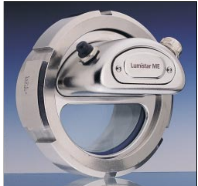
Stainless steel Lumiglas luminaire series Lumistar ME combined with screwed sightglass.
